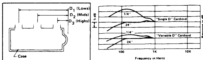
FIGURE 13— "Variable-D" Cardioid Microphone
