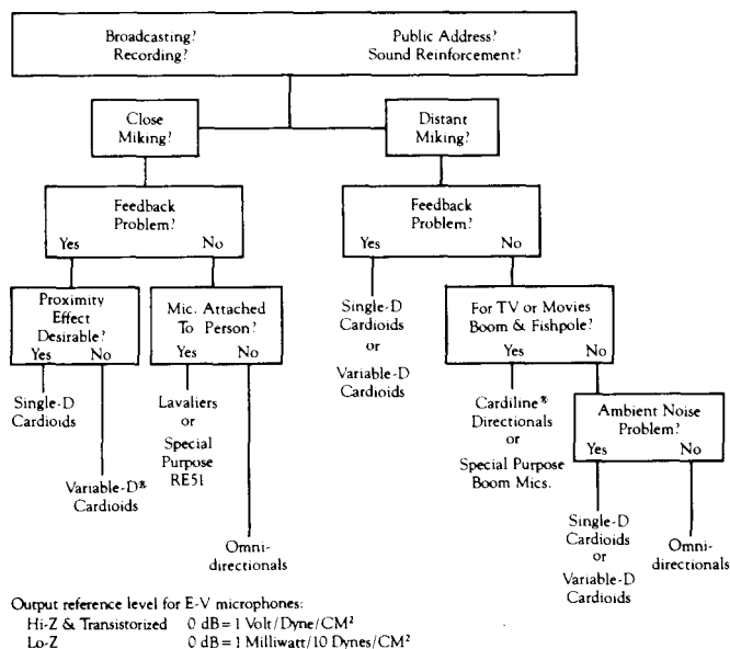
FIGURE 19 - Microphone Application/Recommendation Chart
