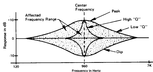
FIGURE 5 - "Q" of a Peak/Dip Equalizer
