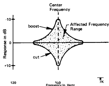
FIGURE 4 - Peak/Dip Equalization Curve
