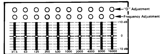
FIGURE 13 - Paragraphic Equalizer
