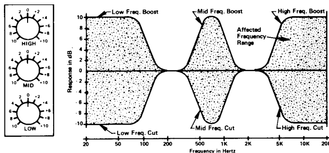
FIGURE 9 - Three Knob (three frequency) Fixed Frequency Equalizer
