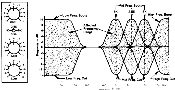
FIGURE 10 - Three Knob (five frequency) Equalizer with Switchable Mid-Range
