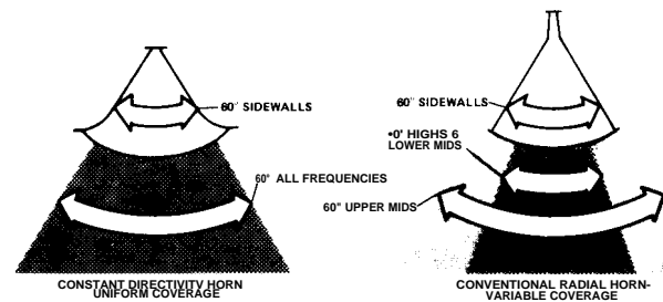
FIGURE 1 - Horizontal (Side-to-Side) Coverage Angle Comparison, Constant Directivity and Conventional Radial Horns
