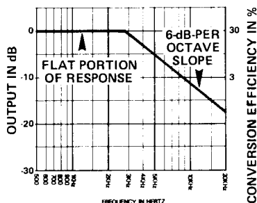
FIGURE 7 - "Newman Criteria" Total Output Reference Standard for Compression Drivers (No Horn)
