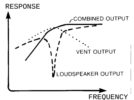
FIGURE 3 - How Loudspeaker and Vent Output Combine in a Vented System
