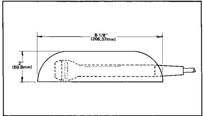
FIGURE 5 Cardioid Microphone in a Mike Mouse
