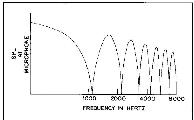
FIGURE 2 Comb Filter Effect
