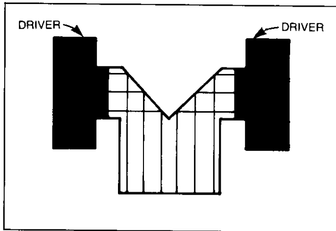
FIGURE 3 Wedge Type Reflective Manifold Showing Rays Coherently Reflected
